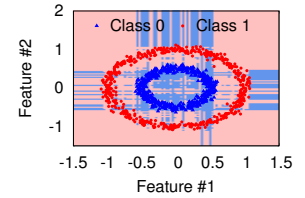
Figure 13: Amazon's decision boundary on CIRCLE.
